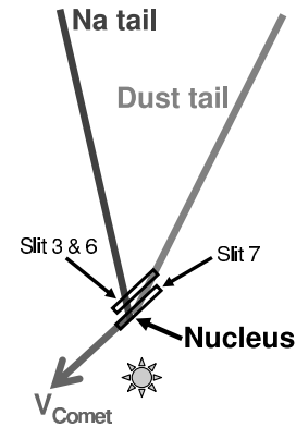
Fig. 1. Cartoon of the observation done by Themis 10 January 2007. The three positions during that observation, namely, slit positions 3, 6, and 7 are displayed in this diagram. The orientations of the sodium tail and of the dust tail have been calculated from the syndyne model (Fulle 2004).
