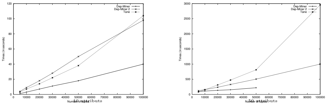
Fig. 6. Execution times (in seconds) for correlated data (50%)
