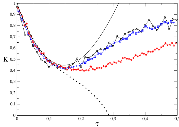
Figure 2. K^*(2\tau) (circles), and the form factors for a (50, 50, 1) quasar graph (squares) and for a (50, 50, 50) quasar graph (stars). The solid line corresponds to the \tau^3 expansion in the \nu_3 = 0, \nu_1 = \nu_2 case, the dashed line corresponds to the \tau^3 expansion in the \nu_1 = \nu_2 = \nu_3 case.
