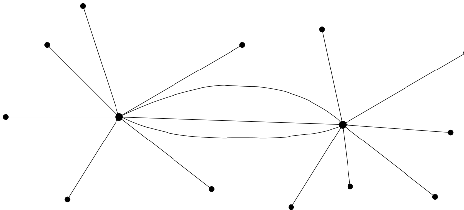
Figure 1. A quasar graph with V_1 = V_2 = 6 and M = 3
