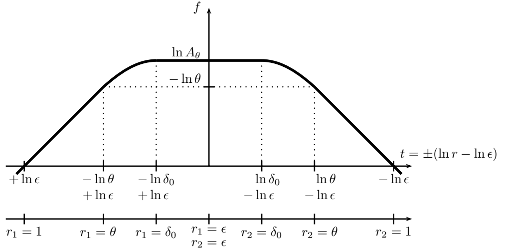
FIGURE 2. The function f
