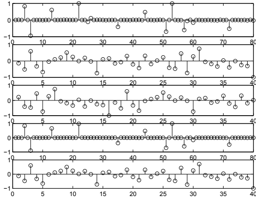
Fig. 2. A sample of our experiments. From top to bottom, first plot represents a randomly generated coefficient vector \alpha , second plot is the synthetic vector s which has the coefficient vector \alpha on the randomly generated dictionary \Phi , third plot is a randomly shifted version of vector s which is the input of our algorithm, fourth plot is the estimated coefficient vector \hat{\alpha} , and the last plot is the vector \hat{s} which has the coefficient vector \hat{\alpha} .
