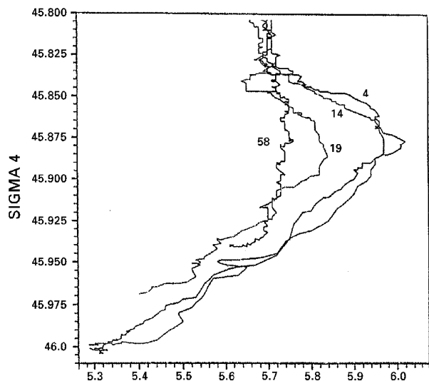
Fig. 13. Evolution of the (a) F-11 ( \text{pmol kg}^{-1} ) and (b) oxygen ( \text{ml}^{-1} ) deep maxima versus \sigma_4 (45.8–46) along the RFZ from Romanche 1 cruise.
