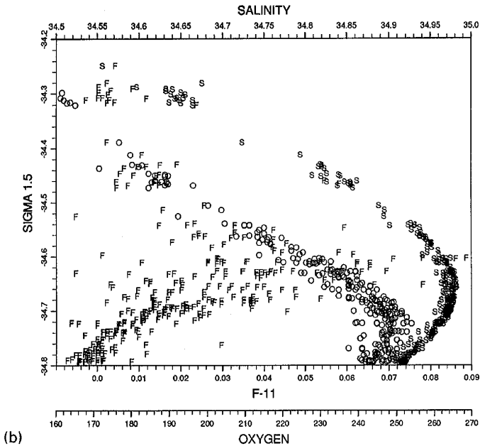
Fig. 11. F-11 ( \text{pmol kg}^{-1} ), salinity and oxygen ( \mu\text{mol kg}^{-1} ) versus \sigma_{1.5} (34.2–34.8) for (a) Romanche 1 stations and (b) Romanche 2 stations.
