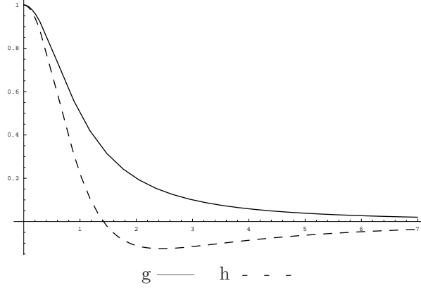
FIGURE 2.2. The diffusion and inverse diffusion weights in the Perona-Malik equation. The diffusion in the direction of level line term coefficient is g(|Du|^2) . See its graph above in continuous line. This term remains positive, which means that there is a diffusion in the direction of the level line, like in the mean curvature motion. This diffusion is slower when the gradient is large. The coefficient of the diffusion in the direction normal to the level line is h(|Du|^2) . This term performs like an inverse heat equation (an enhancement) in the direction of the gradient when the gradient is above a critical value. This enhancement effect also decays when the gradient is large. Compare with the shapes of g and h for the sigma filter.
