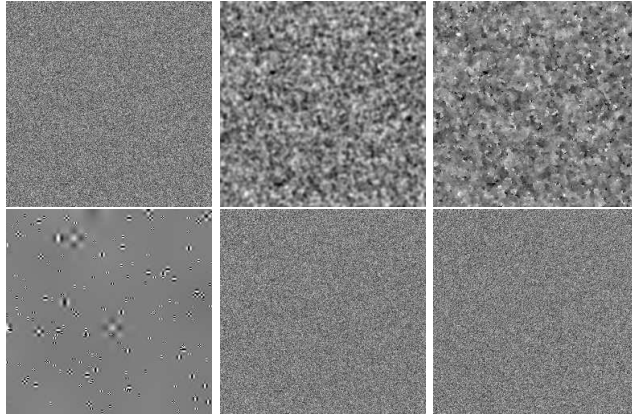
Figure 14: Noise to noise principle: Application of the denoising algorithms to a noise sample. From left to right and top to bottom: noise sample ( \sigma = 15 ), filtered noise by the gaussian filtering, total variation minimization, hard wavelet thresholding, bilateral filter and the NL-means algorithm. The parameters of each algorithm have been tuned in order to have a filtered noise of standard deviation 2.5. For the neighborhood or bilateral filter the research zone has been fixed to 21 \times 21 and for NL-means we have used the whole image. Therefore, only the h parameter has been tuned in order to obtain the desired standard deviation.
