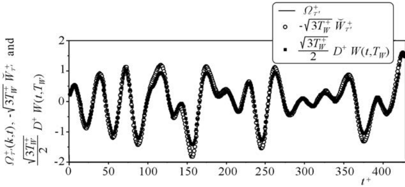
Fig. 7. Comparison of the Mexican Hat transform with the Hilbert transform of WAG and its smoothed time derivative. The raw data is those given in Fig. 5a with T_W^+ = 13
