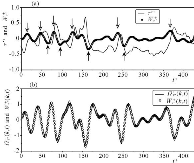
Fig. 5. Sample of instantaneous wall shear stress fluctuations and corresponding wavelet and WAG transforms; (a) instantaneous wall shear stress and its WAG transform in wall units, (b) Mexican Hat transform compared with the WAG induced wavelet transform of the signal shown in (a). The window averaging time and the scale parameter in wall units are respectively T_W^+ = 13 and k^+ = 3/(2T_W^+) = 0.11
