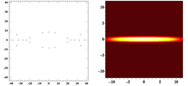
FIG. 2: An example of (a): a configuration of the zeroes (b): density plot. There are only invisible vortices (32 vortices). Here, \nu = 0.48 , \Omega = 0.8767 , \varepsilon^2 = 10^{-3} , G = 3 . The extension in the y direction is given by (8)
