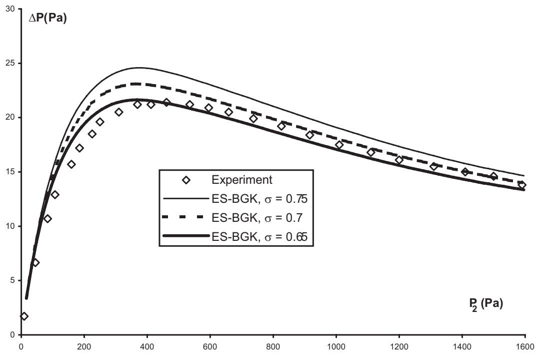
Figure 22. Computed vs. experimental curves of pressure drop in thermal transpiration experiment.
