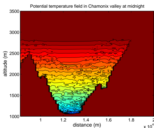
FIG. 3 – Constant contours of the potential temperature field in the Chamonix valley at midnight.
