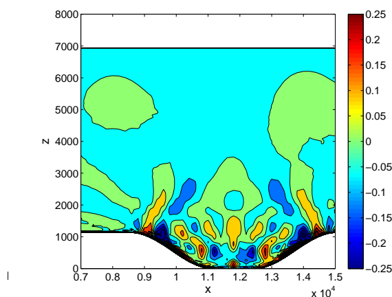
FIG. 1 – Constant contours of the vertical velocity field in a plane perpendicular to the valley axis, at 22 :45 pm.
