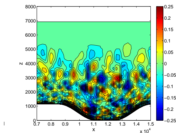
FIG. 2 – Constant contours of the vertical velocity field in a plane perpendicular to the valley axis, at midnight (idealized valley configuration).
