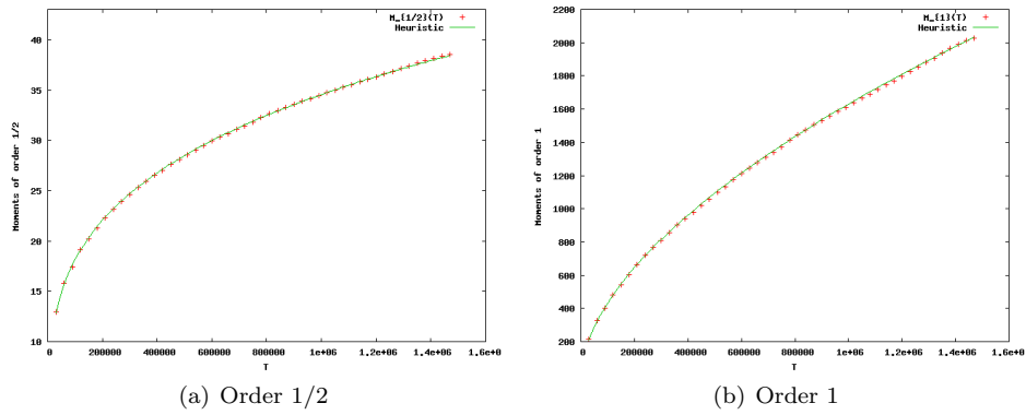
(a) Order 1/2 (b) Order 1 FIGURE 8. Moments of the regulators of the twists of 17a1 by prime discriminants and the functions given by the heuristics.
