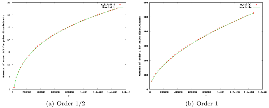
(a) Order 1/2 (b) Order 1 FIGURE 4. Moments of the regulators of the twists of 11a1 by prime discriminants and the functions given by the heuristics.
