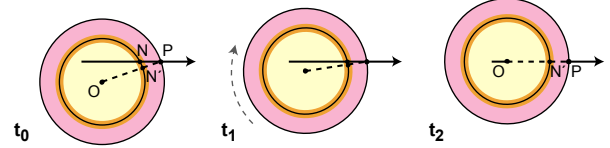
Figure 3: Rotation and translation with momentum over time: like pulling a dinner plate with a string.
