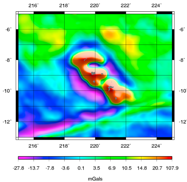
Figure 6. Gravity anomalies computed from the wavelet representation combining gravity anomalies from GGM02S global gravity field and KMS 2002 altimetric grid. Resolution about 35 km; 9651 wavelets are used.
