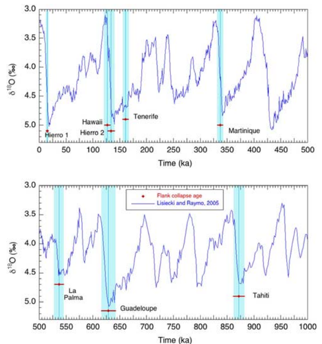
Figure 1. Ages of well-dated oceanic island flank collapses (red diamond) compared with Quaternary climatic changes as shown by a stack of 57 globally distributed δ 18 O records [Lisiecki and Raymo, 2005] (deep blue continuous curve), for the 0–500 and 500–1000 ka intervals. Analytical age uncertainties (1σ) are shown with light blue areas.
