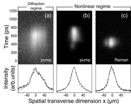
FIG. 3. Experimental spatiotemporal measurements at the waveguide output. (a) The pump pulse with a low input power (1 mW), (b) the pump pulse at high input power (1.74 mW) at the beginning of the trailing edge depletion, and (c) the corresponding first Raman Stokes order pulse. Bottom insets: time-integrated spatial profiles (straight curves) fitted by numerical profiles (dashed curves).
