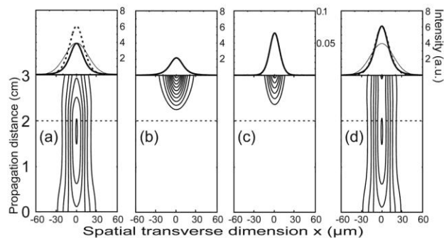
Fig. 1. Numerical simulation of the generation of a three-frequency spatial soliton. Bottom: contour plots of (a) the pump, (b) Stokes, (c) anti-Stokes, and (d) whole beam. Top: transverse beam profiles at the waveguide input (thin solid curve), output (bold solid curve), and after a 2 cm propagation (dashed curve). The parameters are input width = 40 μm, P_{\text{sat}}=0.02 W/m, g_r=23.2 cm/MW. P_p=1.6P_s .
