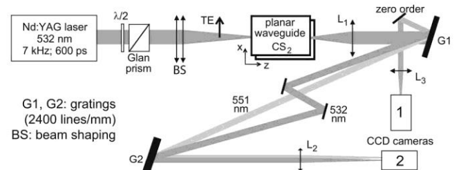
Fig. 3. Experimental setup.
