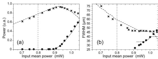
Fig. 4. Experimental (a) output power and (b) FWHM versus input power for the pump ( \times ) and the Stokes ( \bullet ) waves. Dashed curves, numerical results. The vertical dotted lines indicate the fundamental soliton mean power (0.8 mW) for which scalar soliton behavior has been experimentally observed.
