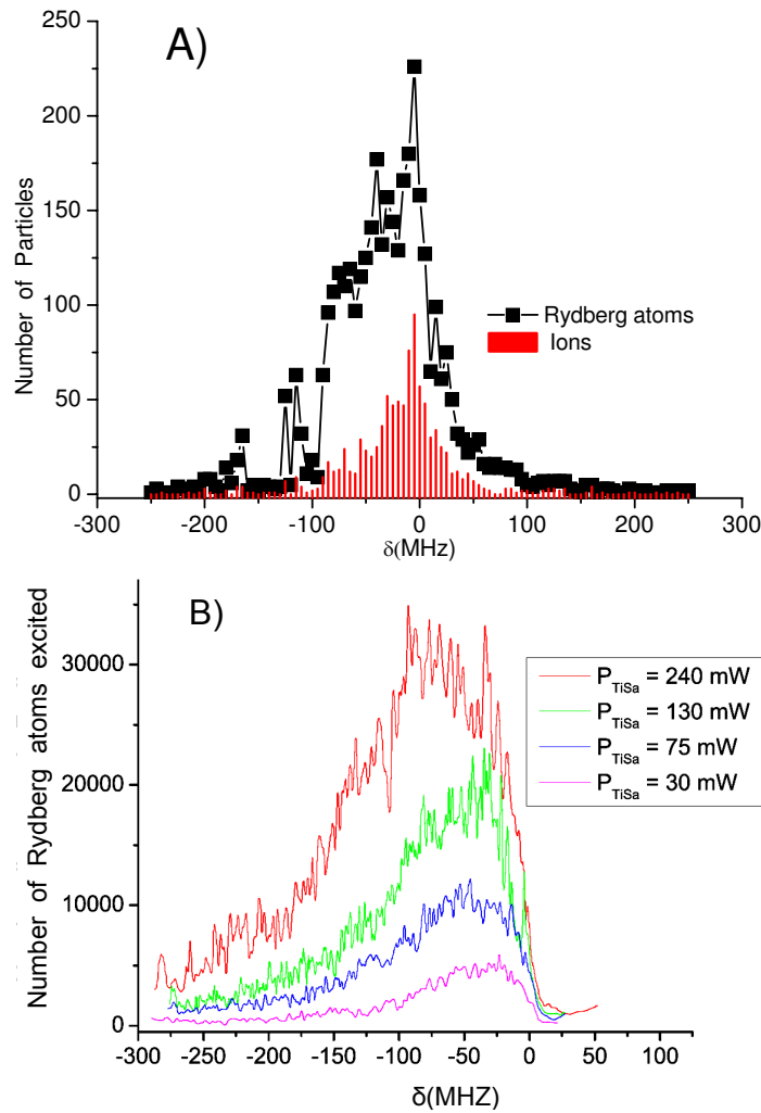
Figure 4. A) Monte Carlo simulation. Number of Rydberg atoms and ions versus the laser detuning. For n = 81 , excitation time 20\mu s , 2000 atoms, D = 2 * 10^{10} cm^{-3} , I=10* I_{sat} . B) Experimental result, see figure 1 B) and [11] for details on the excitation scheme. Number of Rydberg atoms versus the laser detuning in a combined pulsed ( 7ns, 15\mu J ) and cw-excitation (Ti:Sa) at different powers for the excitation of 37p1/2 . Excitation time (Ti:sa) = 400ns .
