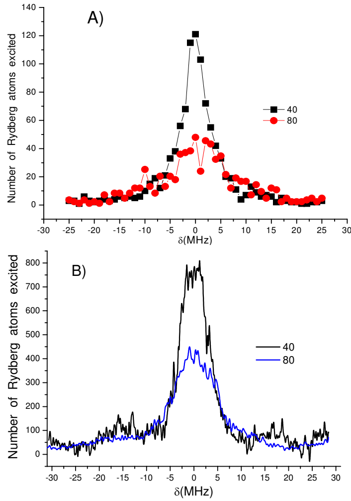
Figure 3. (A) Number of Rydberg atoms excited versus the detuning of the excitation laser for n=40 and 80 . Monte Carlo simulations with 2000 atoms at a density D = 2 * 10^{10} \text{cm}^{-3} and an external electric field of 50 \text{mV/cm} . This result is taken after a laser excitation time of 300 \text{ns} , I=0.7 * I_{\text{sat}} , where I_{\text{sat}} is the saturation intensity of the transition 7s \rightarrow np . The mean number of ions formed during the simulation varies from 0.5 for n=40 to 1.3 for n=80 . (B) Experimental data for n=40 ( P=20 \text{mW} ) and 80 ( P=100 \text{mW} ) at D = 2 * 10^{10} \text{cm}^{-3} , excitation time 300 \text{ns} . The mean number of ions formed per shot is less than 2 .
