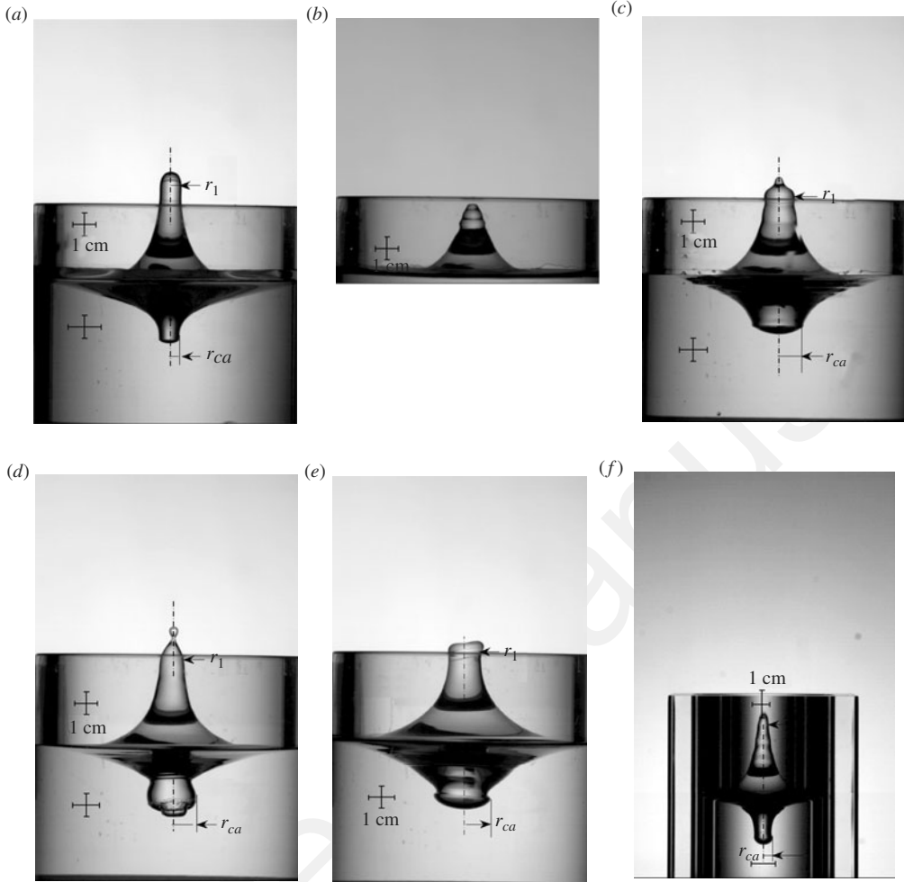
FIGURE 15. Composite images (a, c–e) obtained in container R = 5 cm and image (f) obtained in container R = 2.5 cm, showing the last stable wave amplitude and the following (half a period later) wave depression (cavity) below, for glycerine–water (a), water (c) and FC-72 (d, e). (b) The wave crest for water, with parasitic capillary waves, taken at 0.186 wave period before the maximum wave amplitude is reached, shown in (c); (a) \omega_f/2\pi = 8.85 Hz, A/R = 0.0368 ; (c) \omega_f/2\pi = 8.86 Hz, A/R = 0.0154 ; (d) \omega_f/2\pi = 8.77 Hz, A/R = 0.0179 ; (e) \omega_f/2\pi = 8.35 Hz, A/R = 0.0143 ; (f) R = 2.5 cm, FC-72, \omega_f/2\pi = 11.65 Hz, A/R = 0.0175 .
