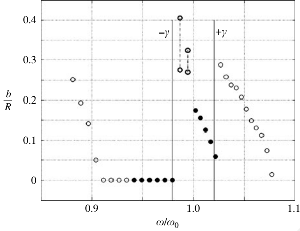
FIGURE 3. Wave-amplitude response for forcing amplitude, A/R=0.006 , indicated by the horizontal dashed line in figure 2. \bullet , steady-state axisymmetric waves; \circ , the range of the wave-amplitude modulation. The dash-dotted vertical lines connecting the same symbols give the magnitude of the amplitude modulations and the thin solid vertical lines indicate the limits -\gamma < \beta < \gamma , equation (5) with \varepsilon=0.023 . \circ , steady-state asymmetric wave motions of modes (2,1) when \omega/\omega_0 < 0.942 and (3,1) above; +\gamma=0.90 .
