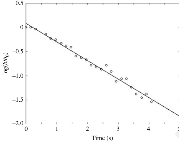
FIGURE 1. Typical decay of the wave amplitude showing the logarithm of b/b_0 as a function of time for \omega = 38.18 \text{ rad s}^{-1} . The experimental points correspond to the wave amplitude at each period and b_0 is the wave amplitude at the stop of the container forcing. The straight line is a least-squares fit and has a slope of 0.39 \text{ s}^{-1} .
