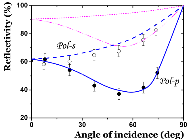
FIG. 2: Simulated reflectivity as a function of angle of incidence for a 250 fs, 248 nm laser pulse for s -polarised (dashed line) and p -polarised (solid line) irradiation of an aluminum target at 10^{14} W/cm 2 intensity. Minimal reflectivity is obtained for an angle of (59 \pm 3)^\circ . Simulations performed with \nu_{neq} = 0 are superposed for s (short-dashed line) and p (dotted line) polarization. Experimental data points (open ( s ) and closed ( p ) circles with error bars) are taken from Fedosejevs et al. [38].
