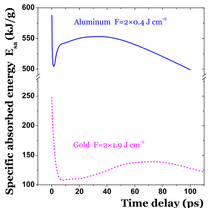
FIG. 6: Calculated specific absorbed energy in the skin depth of an aluminum target irradiated by a double pulse ( 2 \times 0.4 \text{ Jcm}^{-2} ) and a gold target irradiated by a double pulse ( 2 \times 1.9 \text{ Jcm}^{-2} ). Simulations were performed as a function of time delay.
