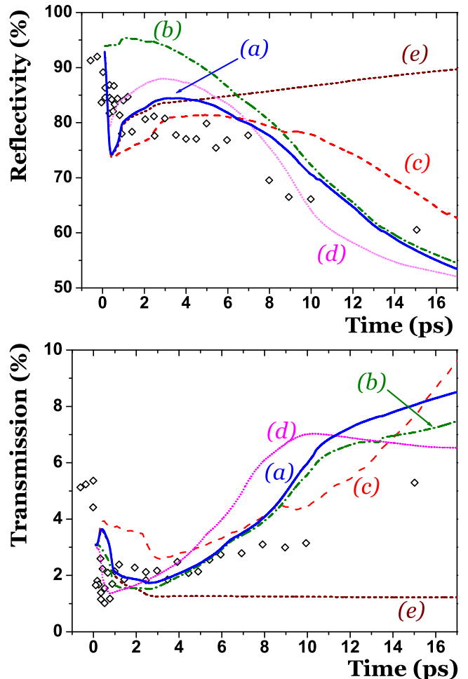
FIG. 4: Numerical evolution (curves) of the reflectivity and the transmission of a 800 nm pulse probing a 28 nm gold foil thickness, for different simulation configurations. The solid line (a) corresponds to the best-fitted complete simulation. The dash-dotted line (b) is a simulation without nonequilibrium contribution in the absorption. The dashed line (c) and the short-dotted line (d) correspond to simulations performed with a lower ( \gamma = \gamma_0/4 ) and a higher ( \gamma = \gamma_0 \times 2 ) e-ph coupling term, respectively. The hydrodynamics processes have been switched off in the simulation shown by the short-dashed line (e). Experimental data points (black diamonds) are taken from Widmann et al [5].
