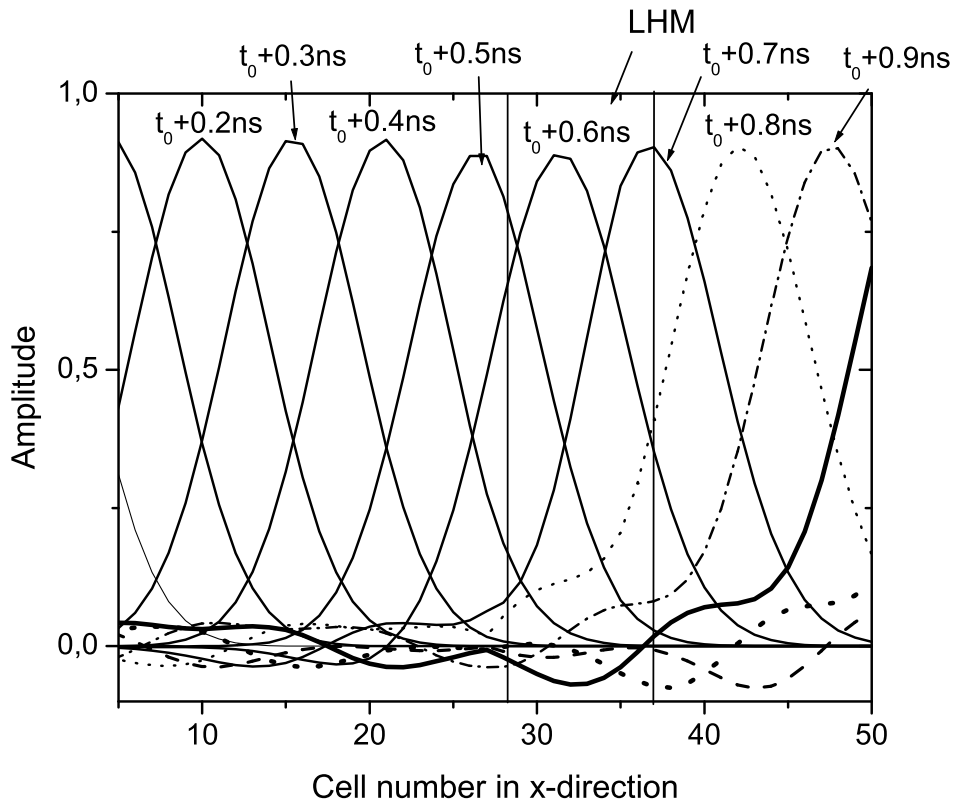
Figure 4: Amplitude of the field versus x -direction at different time instants. The slab width is d = 40\text{ mm} . A plane wave with a gaussian pulse comes from the left side. The position of the LHM is indicated in the figure. Note that the wave appears to propagate in the LHM as in the air (except for a small reflected energy part that is due to imperfection of the matching).
