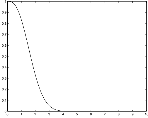
Figure 3: Sequence (\varphi_j^\zeta)_j constructed with (18) for \zeta = 0.76818 .
