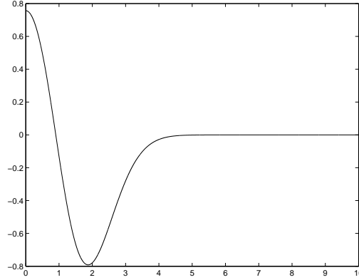
Figure 5: Second eigenvector of H(\zeta) for \zeta close to \zeta_0 .
