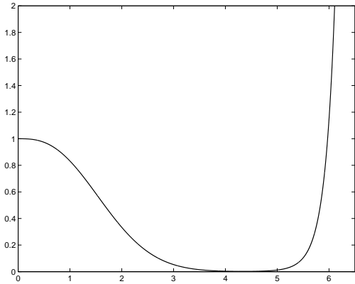
Figure 1: (\tilde{\varphi}_j^\zeta)_j for \zeta = 0.76818 .
