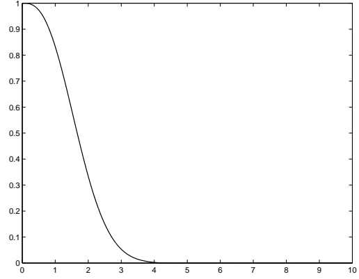
Figure 4: Sequence (\varphi_j^\zeta)_j constructed with (19) for \zeta = 0.76819 .
