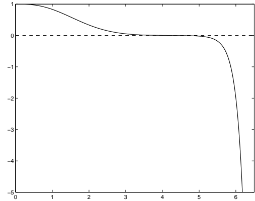
Figure 2: (\tilde{\varphi}_j^\zeta)_j for \zeta = 0.76819 .
