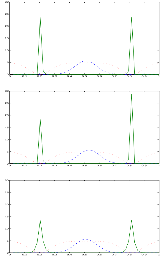
Fig. 1. Evolution of \rho in the 1D-case. Solid line : initial datum, dashed line : final probability, dotted line : potential. Top: symmetric initial probability. Middle: slightly shifted initial probability. Bottom: case \varepsilon^2 = 10^{-2} .
