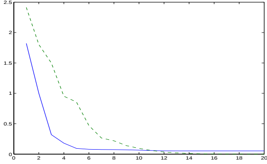
Fig. 2. Numerical convergence in the 20 first iterations. Solid line : Values of E_{dt,dx} . dashed line : values of the termination criterion defined in (18) (rescaled).
