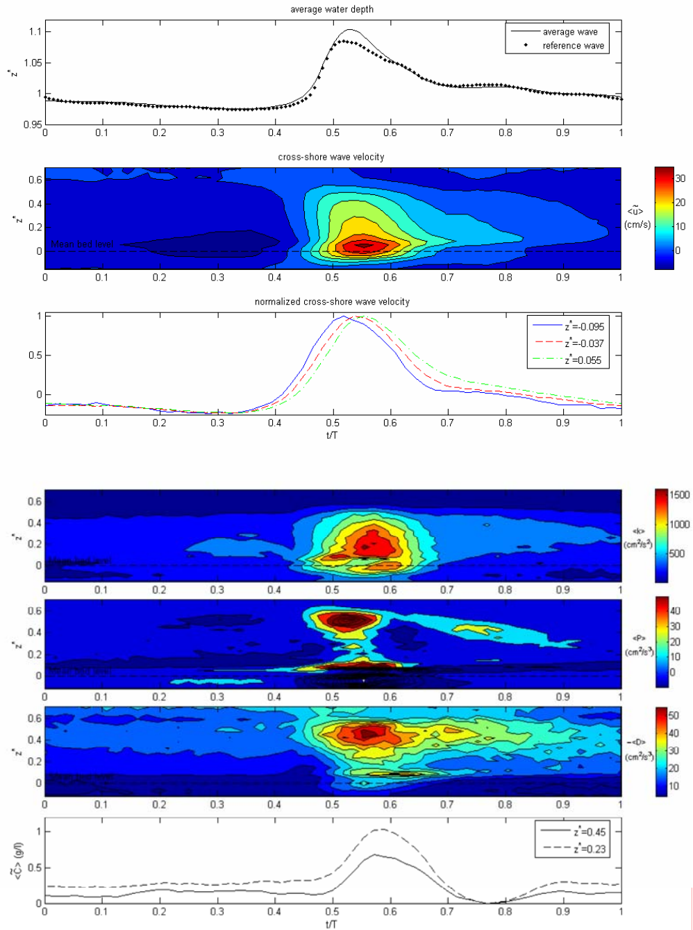
Figure 4. Measurements at x=12m of (a) surface elevation (b) cross-shore wave velocity field, (c) normalised cross-shore wave velocity at three depths, (d) TKE field, (e) TKE production field, (f) TKE dissipation rate field, (g) sediment concentration (wave component) at two depths.
