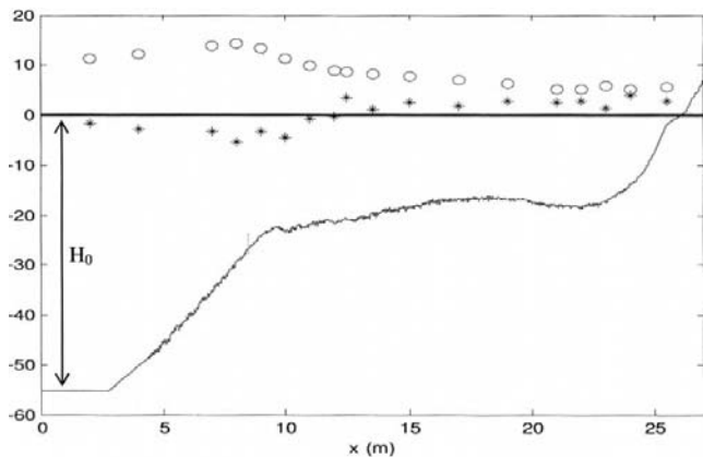
Figure 1. Cross-shore profile of bottom elevation at equilibrium, mean free-surface elevation \bar{\eta} in mm (set-down and setup: *) and H_{rms} in cm (o) for H_0=53\text{cm} .
