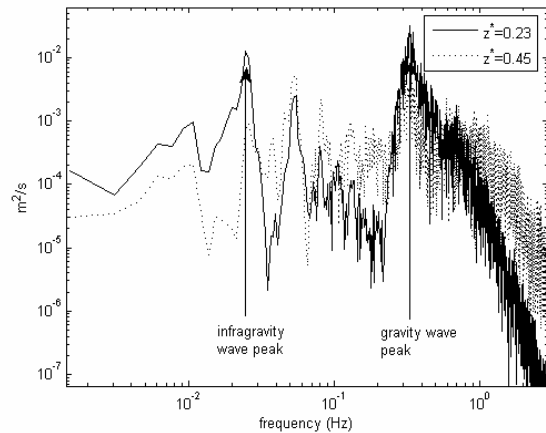
Figure 6 Velocity spectra of cross-shore wave velocity at average wave breaking point ( x=12m )
