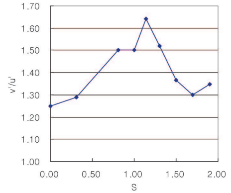
Fig. 10 Variation of anisotropy as S changes at y=10\text{mm} on the centerline.
