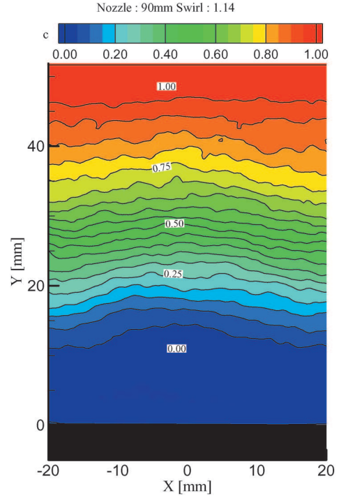
Fig. 17 Two-dimensional distribution of progress variable
