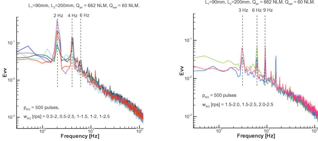
Fig. 7 Effect of random rotating speed under constant short period condition. (left) \omega_{AG}=0.5-2.0, 0.5-2.5, 1.0-2.5, 1.0-1.5, 1.0-2.0, 1.0-2.5 ; (right) \omega_{AG}=1.5-2.0, 1.5-2.5, 2.0-2.5 . The data are taken at the location, y=10\text{mm} on the center line.
