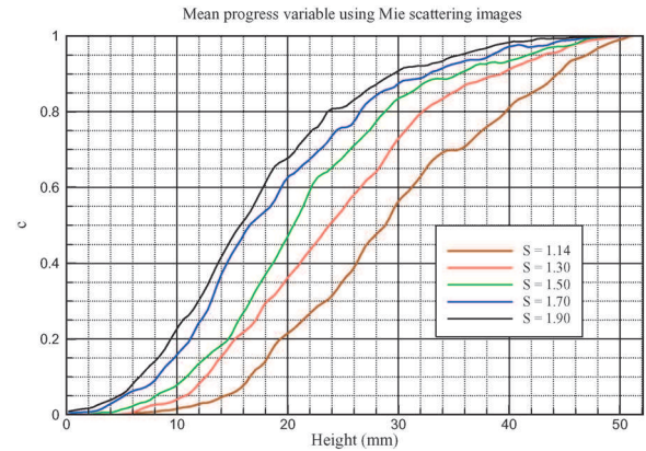
Fig. 18 Mean progress variable for different swirl ( L=90\text{mm} )
