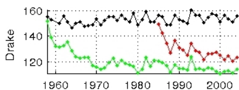
Fig. 9: Mean transport (in Sv) at Drake passage in hindcasts G70, KAB001, and KAB002.
