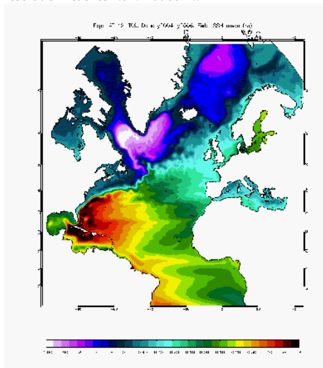
Fig. 2. The NATL12 domain (1615×1585×50 grid points with partial step) and the 2004-2006 mean SSH (in meter) from a hindcast started in 1998 (MERCATOR-Océan).
