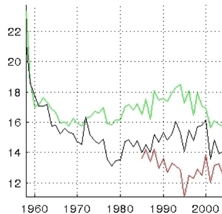
Fig. 7: Variation of the AMOC maximum in the North Atlantic in hindcasts G70, KAB001 and KAB002.
