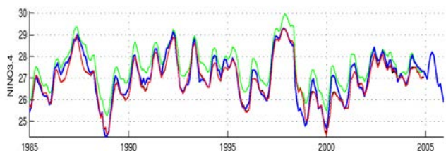
Fig. 8: Time evolution of the ocean surface temperature (°C) in the Niño Box 3-4 in hindcasts G70, KAB001, KAB002 and NOAA observations. Curves for the KAB runs are almost identical.
