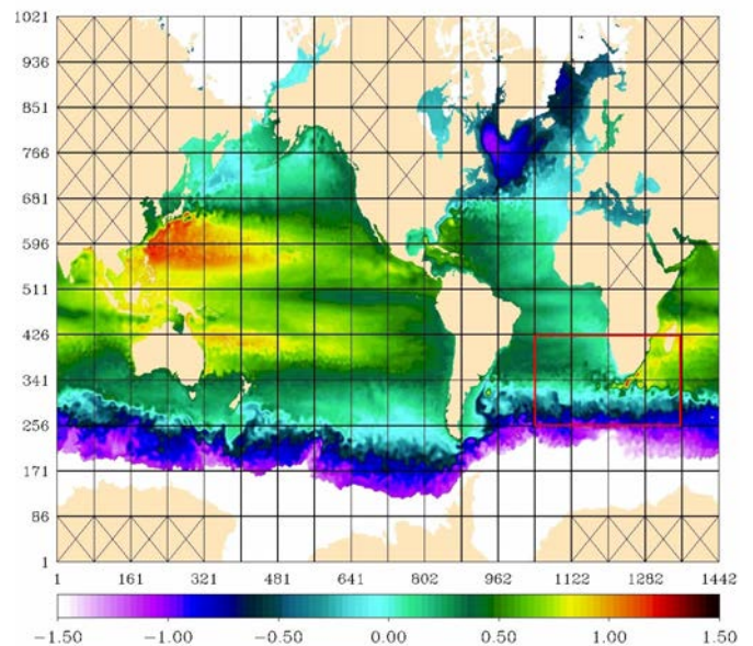
Fig. 1: ORCAii global configurations. The model domain and land-sea mask are shown for the 1/4° ORCA025 configuration (axes correspond to grid points). Colours show a SSH snapshot (in meter) on June 24, 1998 from one of the hindcast runs (G70), sea-ice cover being in white. Boxes show the domain decomposition on a large number of processors, ocean processors (not marked by a cross, 186 of those) being the only ones retained in the calculation. On vector computers a more moderate parallelization (typically up to 32 processors) is used. The red box is the region where a 2-way grid refinement at 1/10-1/12° is being implemented.
