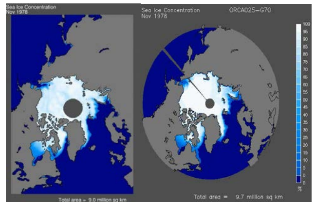
Figure 6: Monthly mean sea-ice concentration and total area in November 1978 (left) from satellite observations and (right) from the G70 hindcast.
