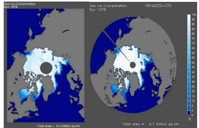
Fig. 6: Monthly mean sea-ice concentration and total area in November 1978 (left) from satellite observations and(right) from the G70 hindcast.
