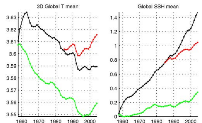
Fig. 3: Evolution of global ocean average temperature and sea level in G70, KAB001 and KAB002.
