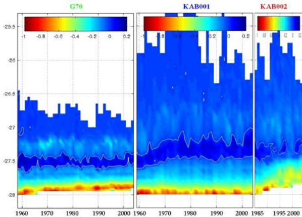
Figure 5: Evolution of the annual mean transport (in Sv) by density classes across the Denmark Strait. Negative values indicate a flow from the Nordic Seas into the Atlantic. The zero contour line is shown in white.
