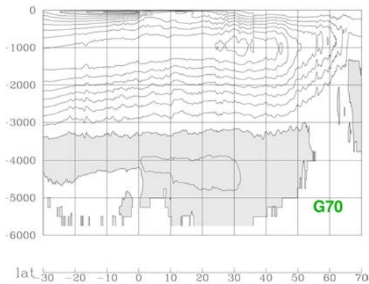
Figure 4: Mean (1990-2004) AMOC in the North Atlantic for hindcast G70. Negative values are shaded grey and contour interval is 2 Sv.
