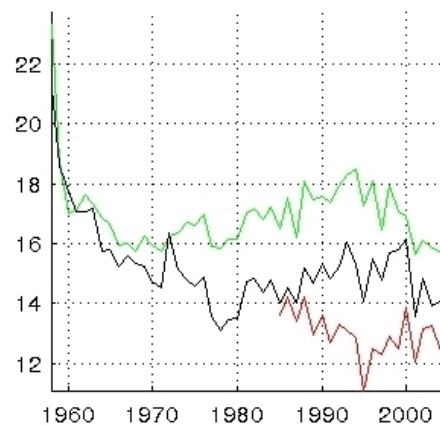
Figure 7: Variation of the AMOC maximum in the North Atlantic in hindcasts G70, KAB001 and KAB002.
