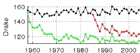
Fig. 9: Mean transport (in Sv) at Drake passage in hindcasts G70, KAB001, and KAB002.
