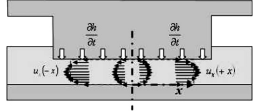
Fig. 3. Definition of the fictive volume for flow rate evaluation.
