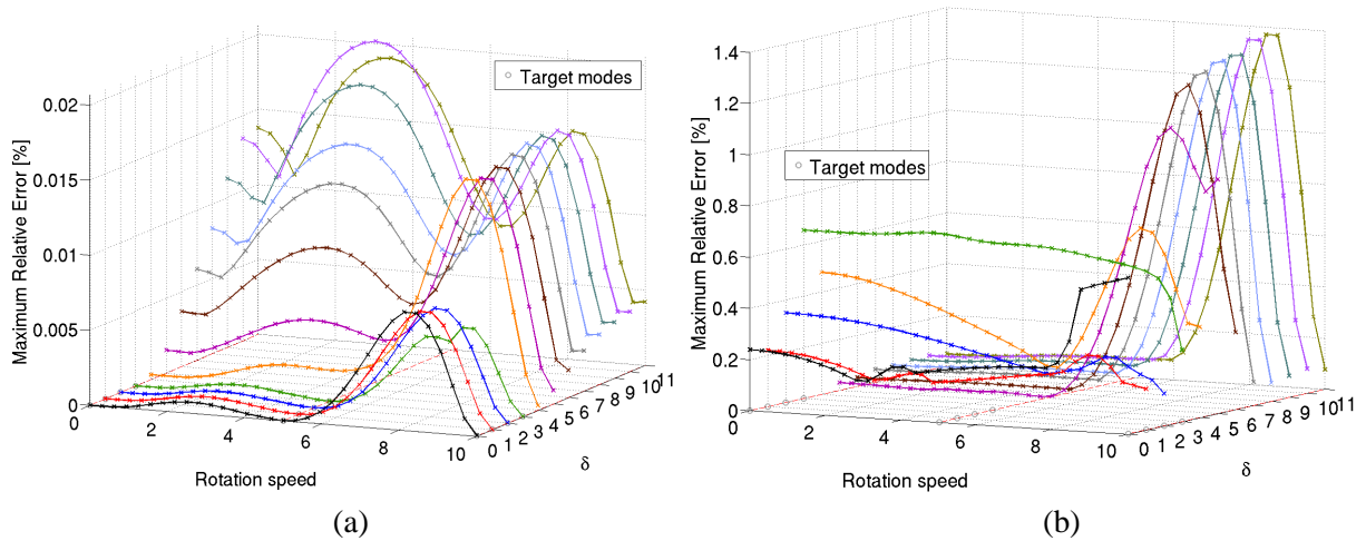
Figure 10: Maximum frequency error for a multi-model built from a QC disk model in the frequency band (a) [1, 5] – (b) [1, 15]
