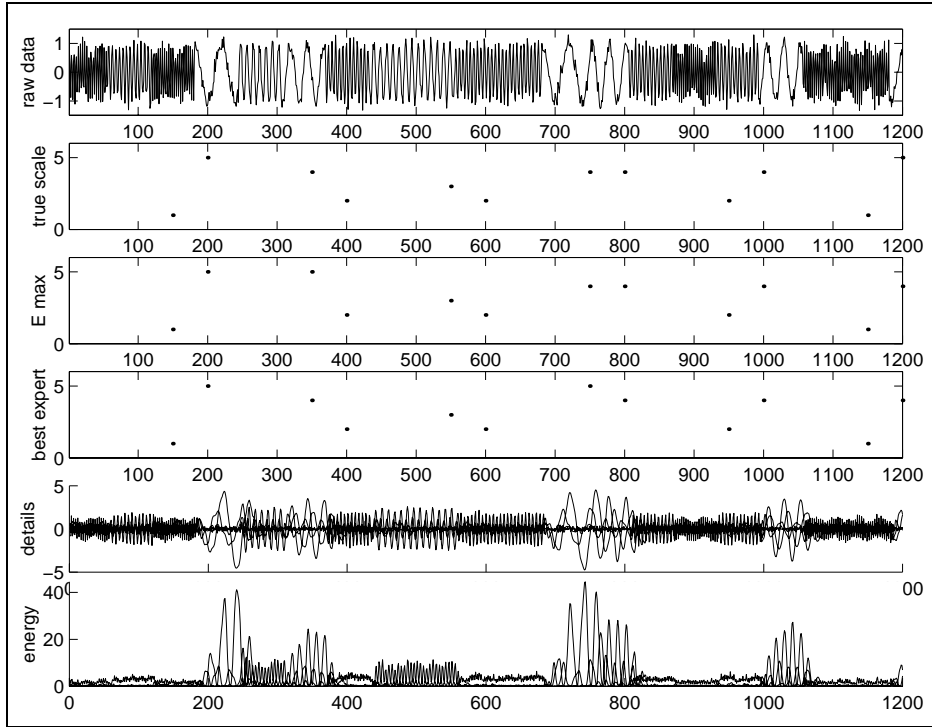
Fig. 1: Random succession of five noisy sine functions. From top to bottom : the raw signal, the true dynamical mode, the scale having maximum energy, the optimal sequence of experts, the wavelet coefficients d_j^t up to scale 6, and the energy estimates.
