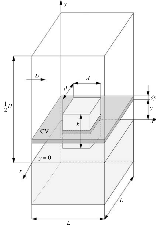
FIGURE 8. Numerical model. Three-dimensional view of the computational domain.
