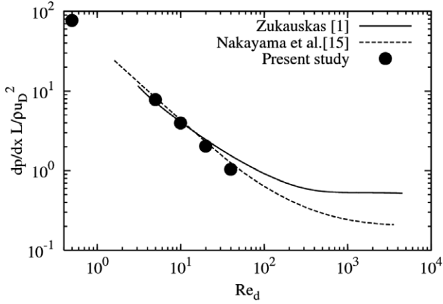
Fig. 5. Dimensionless pressure gradient across the bank of rods. Comparison with Nakayama and Zukauskas results. Aligned arrangement. \varepsilon = 0.875 .
