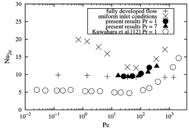
Fig. 6. Constant temperature heating. Comparison of the numerical results with two extreme cases of heat transfer in channel flow.
