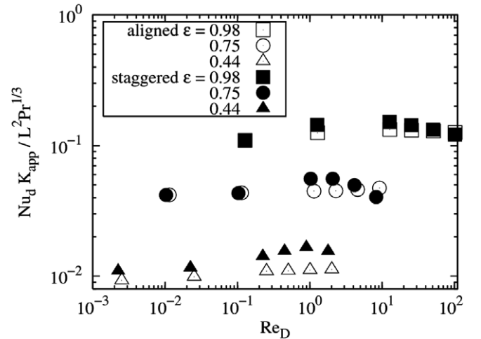
Fig. 12. Thermal performance. Comparison between aligned and staggered arrangements for Pr = 7 .
