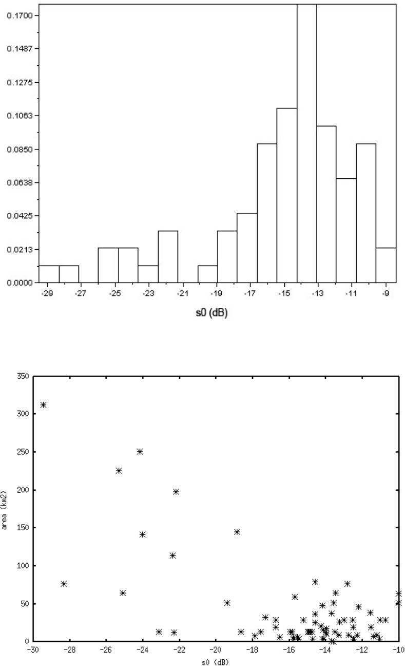
Figure 3. Top: Histogram of \sigma_0 distribution for the 77 lakes, showing two main groups: “bright lakes” with \sigma_0 higher than -19 dB and “dark lakes” with \sigma_0 lower than -22 dB. Bottom: Plot of T16 lake area (in \text{km}^2 ) versus mean \sigma_0 (in dB): smaller lakes are also the brightest, while larger ones are the darkest, with a limit between the two groups around -19/-22 dB.
