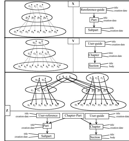
Fig. 16 Representation of the subdatabases X, Y and Z
