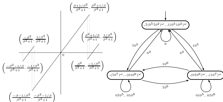
Figure 15. Branching transformation and corresponding automaton, \beta^3 = \beta + 1 .
