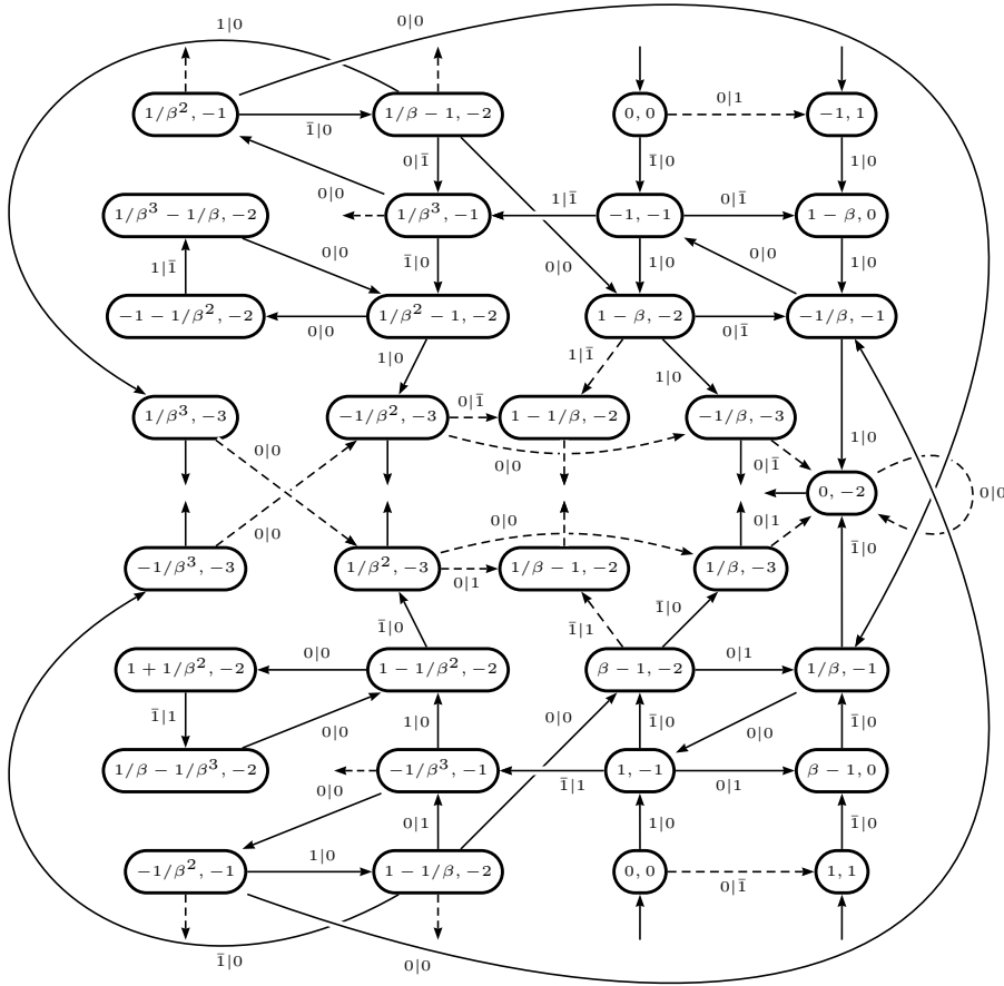
Figure 8. The relevant part of \mathcal{S}_\beta(1) , \beta^3 = \beta^2 + \beta + 1 , and \mathcal{S}_T(1) .
