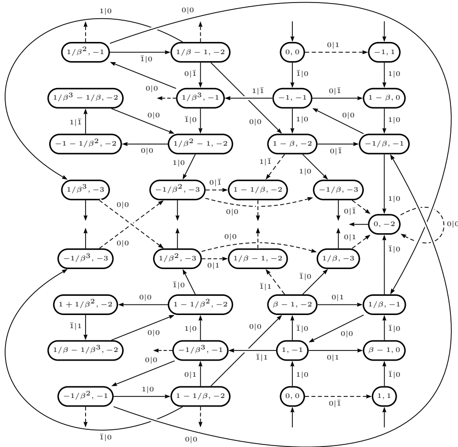
Figure 8. The relevant part of \mathcal{S}_\beta , \beta^3 = \beta^2 + \beta + 1 , and \mathcal{S}_T .
