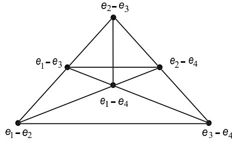
Figure 3: Chambers of A_3
