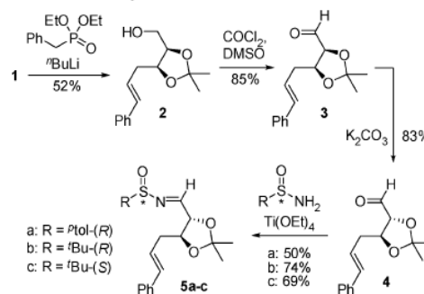
Scheme 2. Synthesis of Chiral Sulfinimines 5a–c
