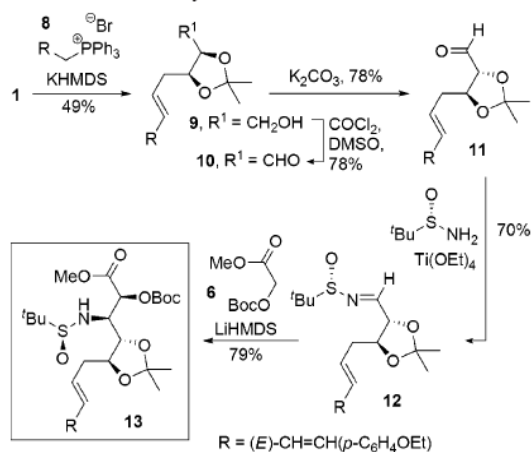
Scheme 3. Synthesis of Protected AETD 13
