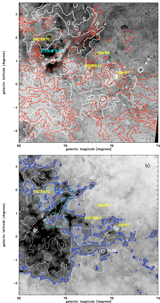
Fig. 5. a) Inverted H_{\alpha} image (courtesy of William McLaughlin) of the Cygnus X south region. Overlaid are white contours of IRAS 100 \mu\text{m} emission (levels 50, 300, 500, 2000, 4000, 5000 MJy/sr) and red contours of ^{12}\text{CO } 1 \rightarrow 0 emission (levels 0.5, 1.5, 3, 5, 7, 9 \text{K km s}^{-1} in the velocity range 6 to 20 \text{km s}^{-1} ) taken from the Center for Astrophysics CO-survey (Dame et al. 1987). b) Extinction map of the same region in grey scale ( A_v = 0 to 10^m ). This map was obtained from the reddening of J - H and H - K colors using 2MASS data (Bontemps et al. 2007, in prep.). The A_v = 5^m contour is outlined in bold blue. Overlaid are the same white contours of IRAS 100 \mu\text{m} emission. The dashed light blue polygon indicates the H II region IC 1318 b/c. Known star clusters are indicated in yellow in both plots.
