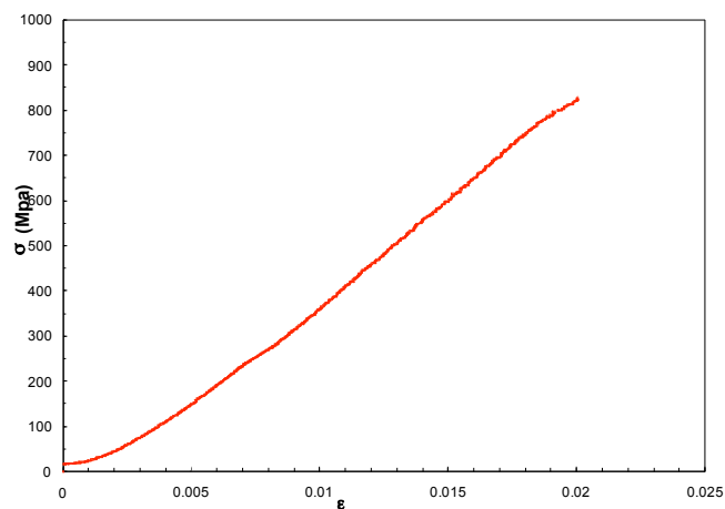
Figure 20: Stress-strain curve of the and (Mg_{65}Cu_{25}Gd_{10})_{97}Fe_3 samples at 300K.
