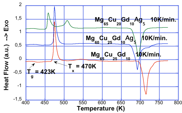
Figure 7: DSC trace for the Mg_{65-x}Cu_{25-y}Gd_{10} alloys.
