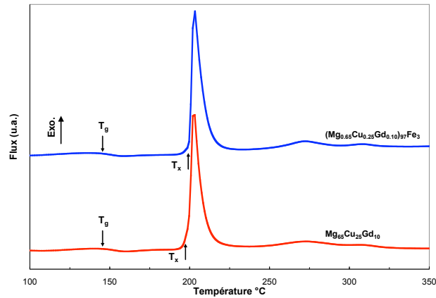
Figure 19: DSC traces of the Mg_{65}Cu_{25}Gd_{10} and (Mg_{65}Cu_{25}Gd_{10})_{97}Fe_3 samples.
