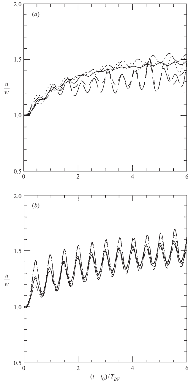
FIGURE 1. Ratio u/w of the horizontal and the vertical r.m.s. values of the velocity components. (a) DNS and (b) EDQNM 2 results for: —, run R2; ···, run R1; ----, run A; — — — —, run B; - · - · - ·, run r2.
