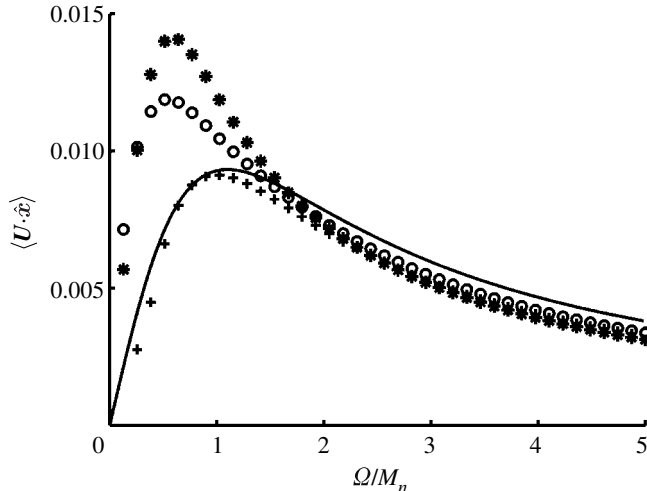
Figure 5. Comparison of the asymptotic expression for swimming in the M_n \rightarrow \infty limit (solid curve) with numerical simulation of the fully nonlinear equations of motion (3.3a)–(3.3d). Asterisks, M_n = 10 ; open circles, 50; crosses, 100 to the M_n \rightarrow \infty asymptotic limit (solid curve) (4.13). b_0 = 1 , and other material parameters are assigned typical values from experiment (3.10).
