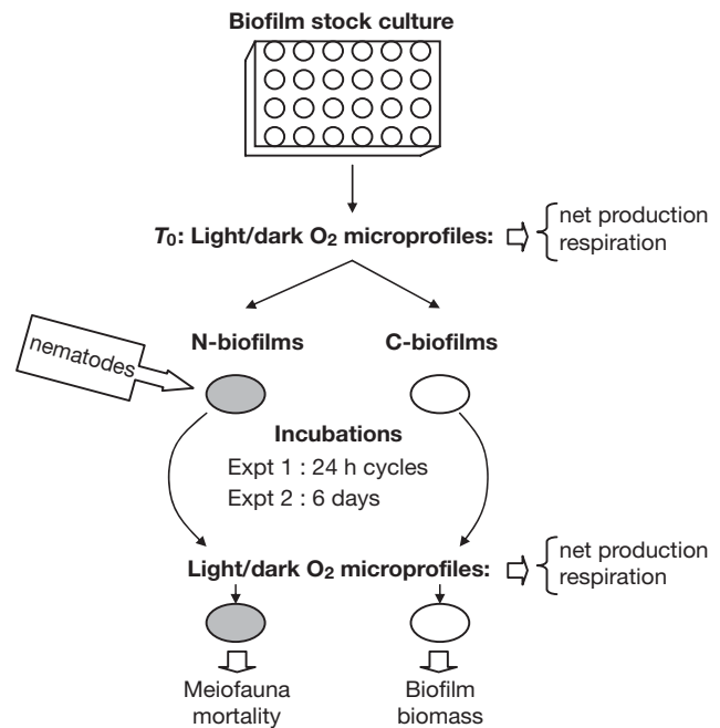
Fig. 1. Experimental designs of both the short-term (24 h) and medium-term (6 d) experiments. T_0 : beginning of incubation period; N-biofilm: with nematodes; C-biofilm: without meiofauna
