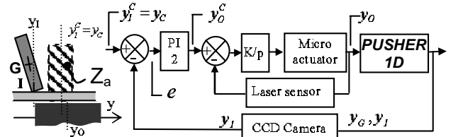
Fig. 13. Coarse controller.
