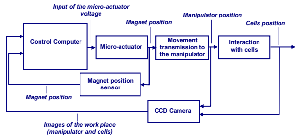
Fig. 3. Information transmission in the experimental device.
