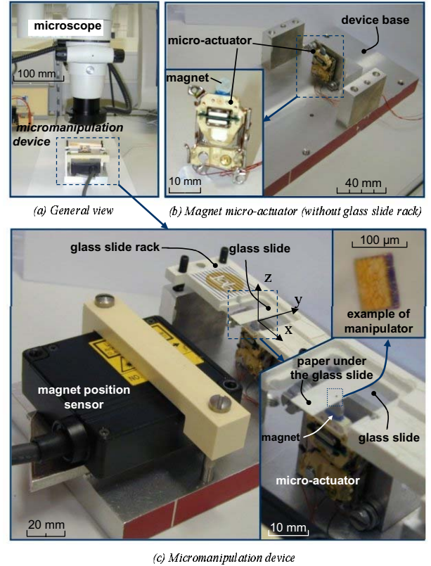
Fig. 2. Experimental device.
