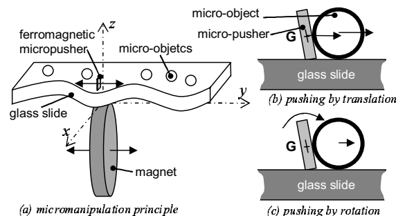
Fig. 1. Micromanipulation principles
