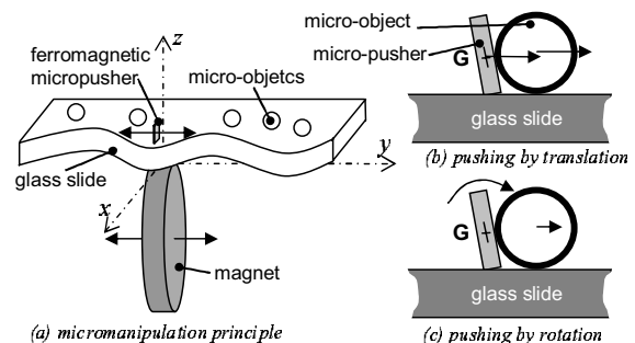
Fig. 1. Micromanipulation principles
