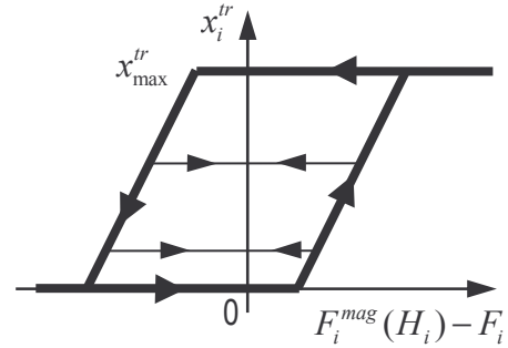
Fig. 4: Hysteresis behaviour due to the martensite reorientation.
