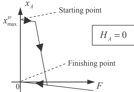
Fig. 5: Displacement of MSM_A when no magnetic field is applied.
