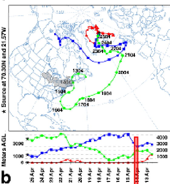
a Backward trajectories ending at 12 UTC 25 Apr 05
