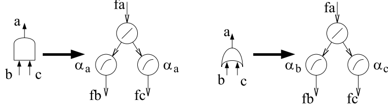
Fig. 4. Transformation of AND and OR gates into a neuro-fuzzy architecture
